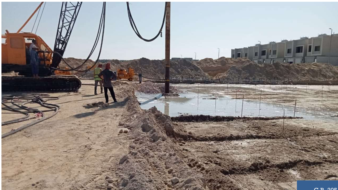
Soil Improvement (Stone Column) work For SWCC Project @ Al Khobar
