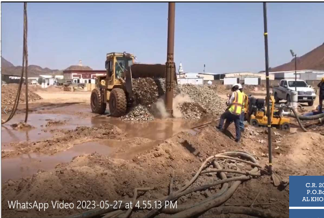
Soil Improvement (Stone Column) work For ISTP -3 PROJECT @ Madinah (Client ACCIONA JV TAWZEA, OWNER – SWCC)
